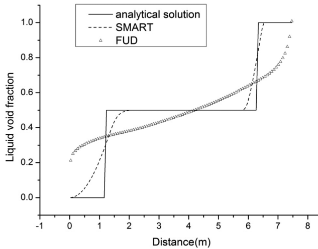
(a) Liquid void fraction
