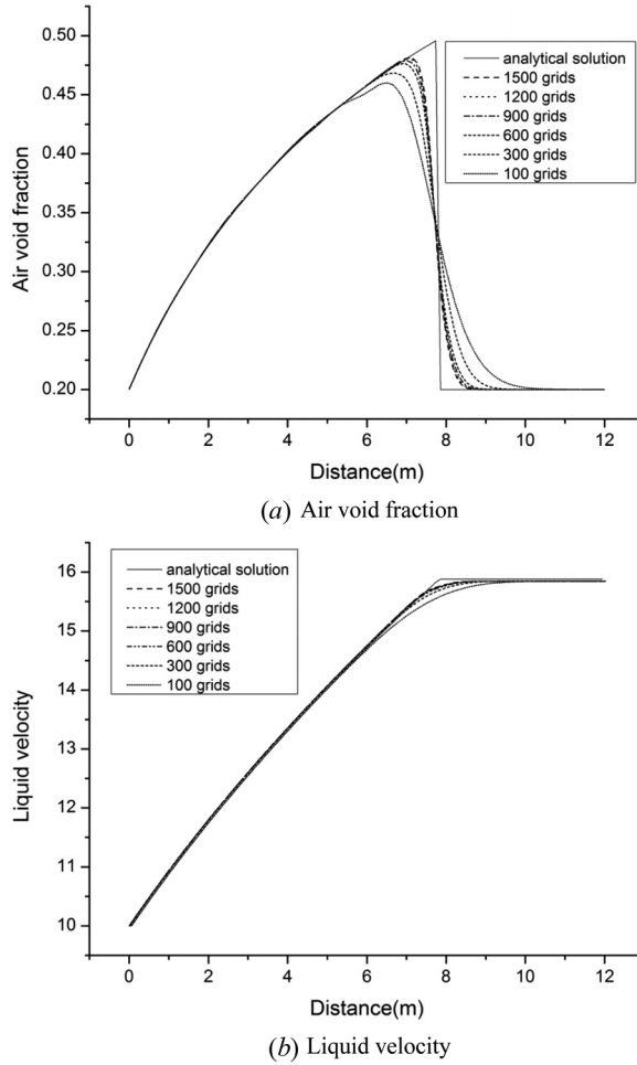
Figure 3. Water faucet problem (time t=0.6 s); grid convergence study; (a) air void fraction and (b) liquid velocity.
