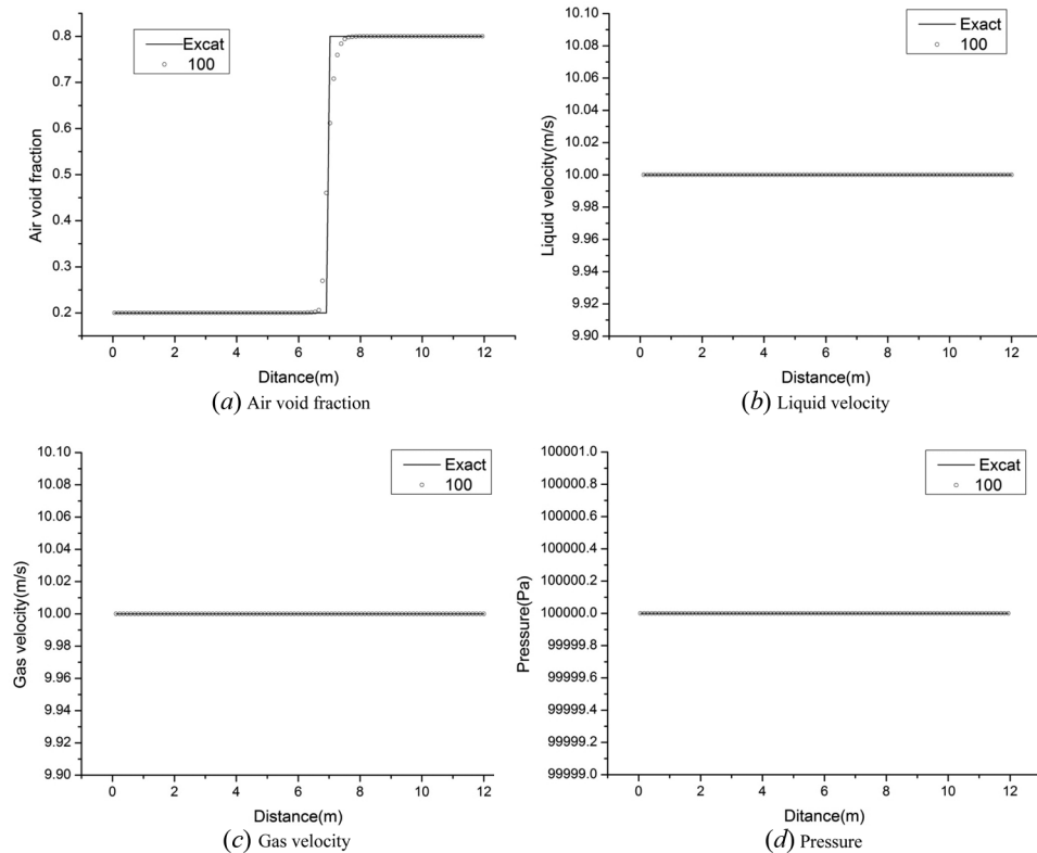
Figure 5. Discontinuity movement in a uniform two-phase flow: (a) air void fraction, (b) liquid velocity, (c) gas velocity, and (d) pressure.
