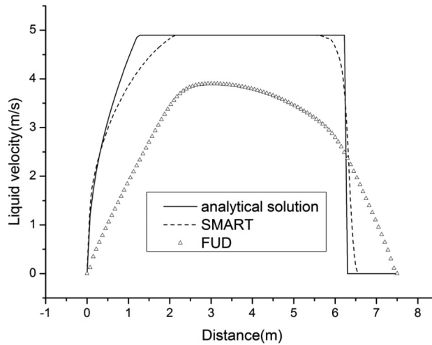
(b) Liquid velocity
