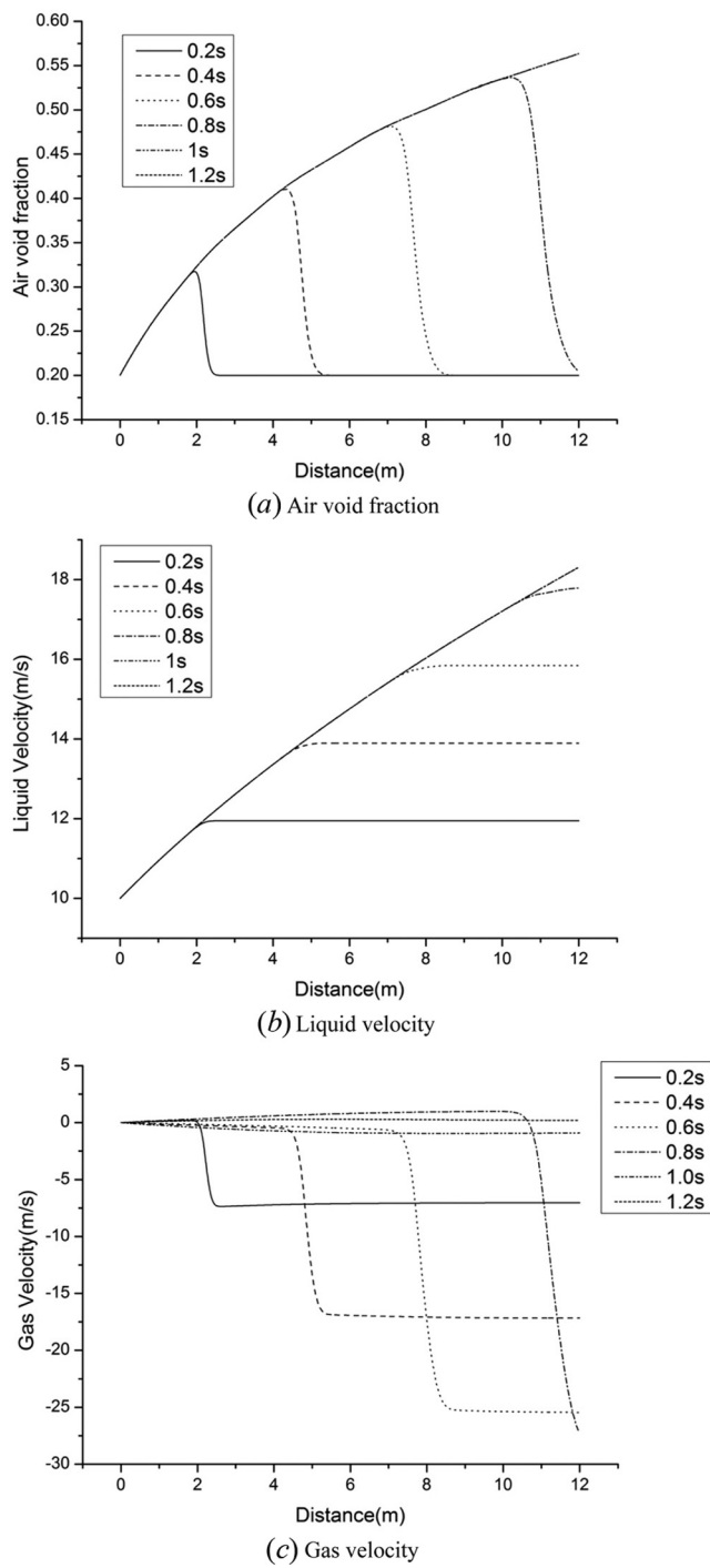
Figure 4. Water faucet problem—time evolution study: (a) air void fraction and (b) liquid velocity.
