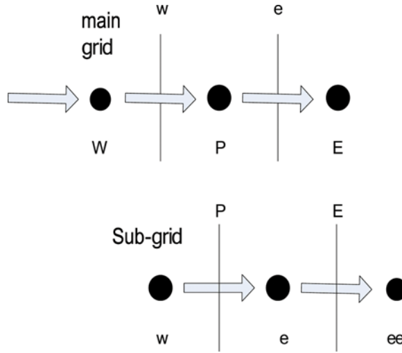
Figure 1. Staggered grid arrangement.
